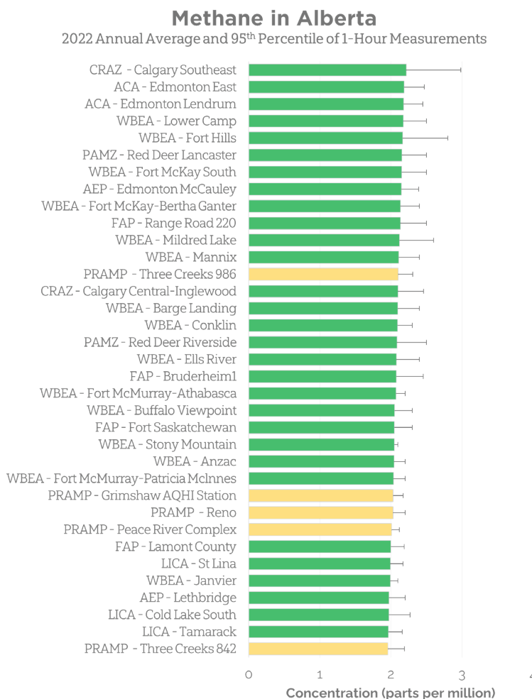
Figure 5: 2022 Methane in Alberta
