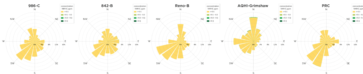
Figure 13: 2022 Hourly non-methane hydrocarbon concentration wind roses
