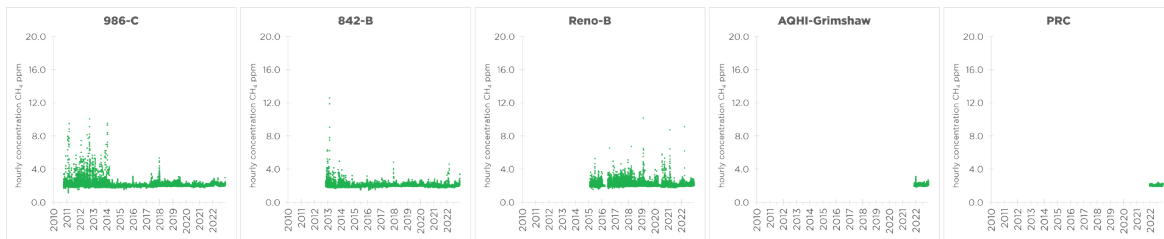
Figure 8: 2010-2022 Hourly methane concentrations
