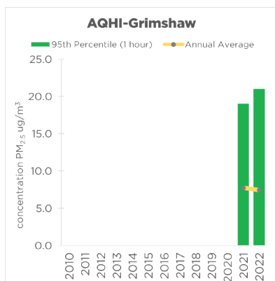
Figure 51: 2010-2022 Annual averages and 95 th percentile of hourly measurements of particulate matter
