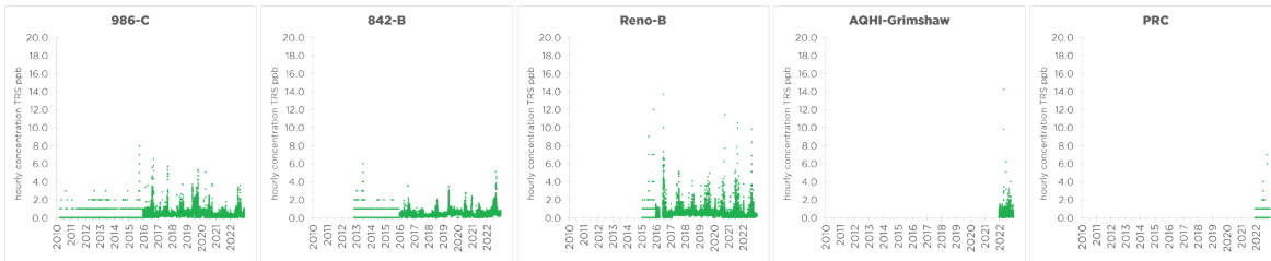
Figure 26: 2010-2022 Hourly total reduced sulphur compounds concentrations
