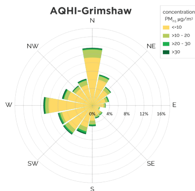
Figure 52: 2010-2022 Hourly particulate matter concentration wind rose
