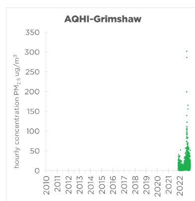
Figure 50: 2010-2022 Hourly particulate matter concentrations
