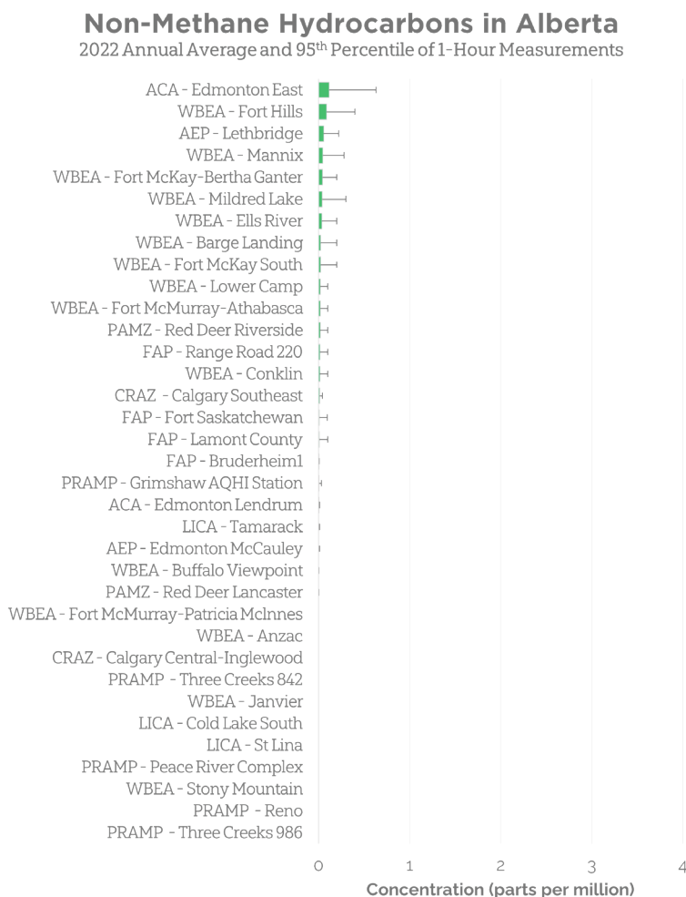
Figure 11: 2022 Non-methane hydrocarbons in Alberta
