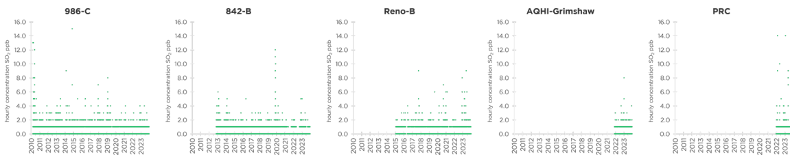
Figure 20: 2010-2023 Hourly sulphur dioxide concentrations
