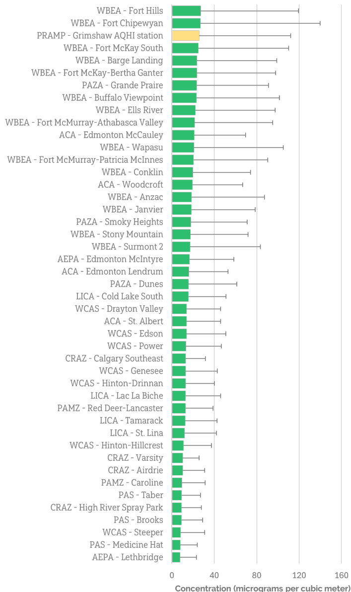
Figure 47: 2023 Particulate Matter in Alberta
