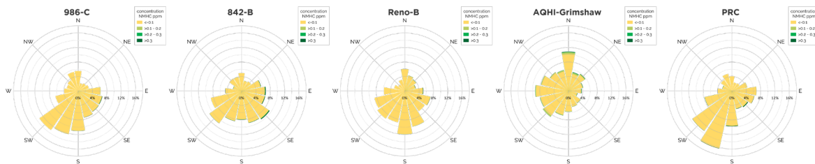
Figure 13: 2023 Hourly non-methane hydrocarbon concentration wind roses
