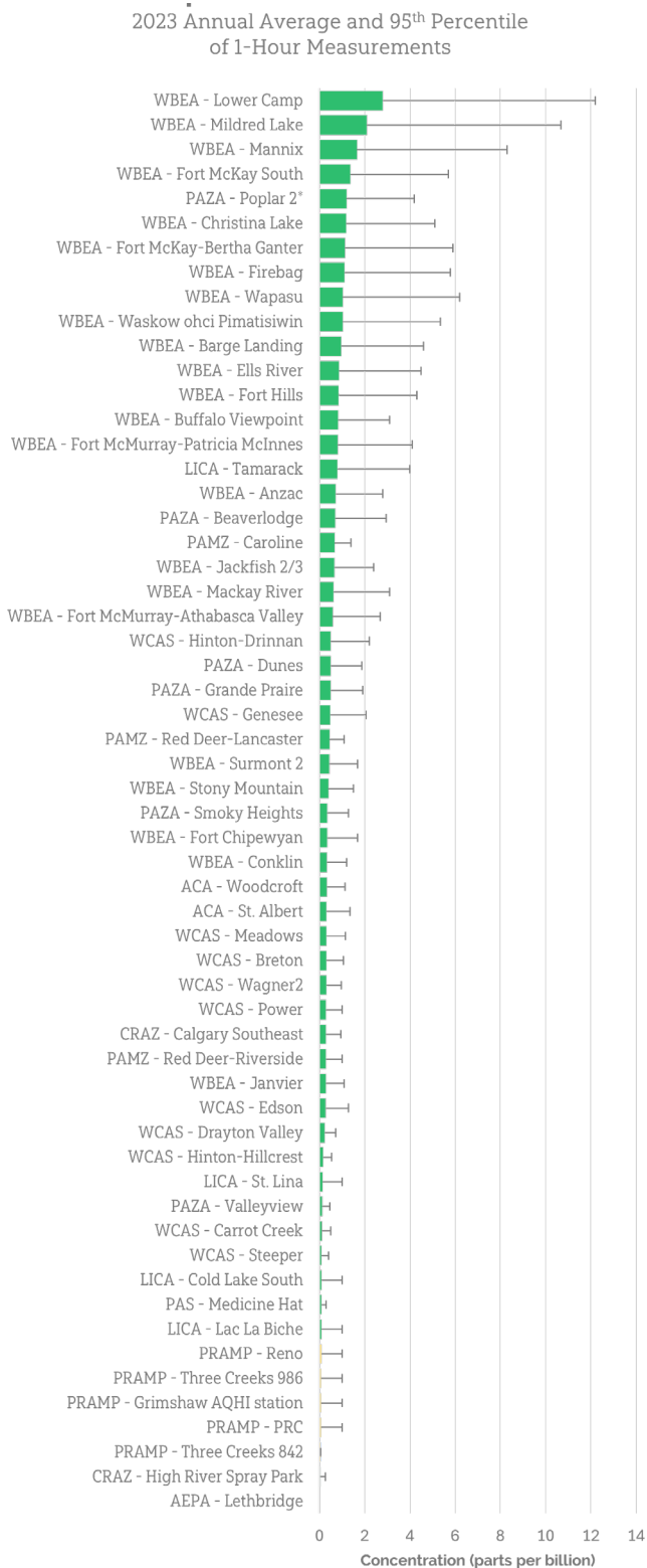
Figure 17: 2023 Sulphur dioxide in Alberta
