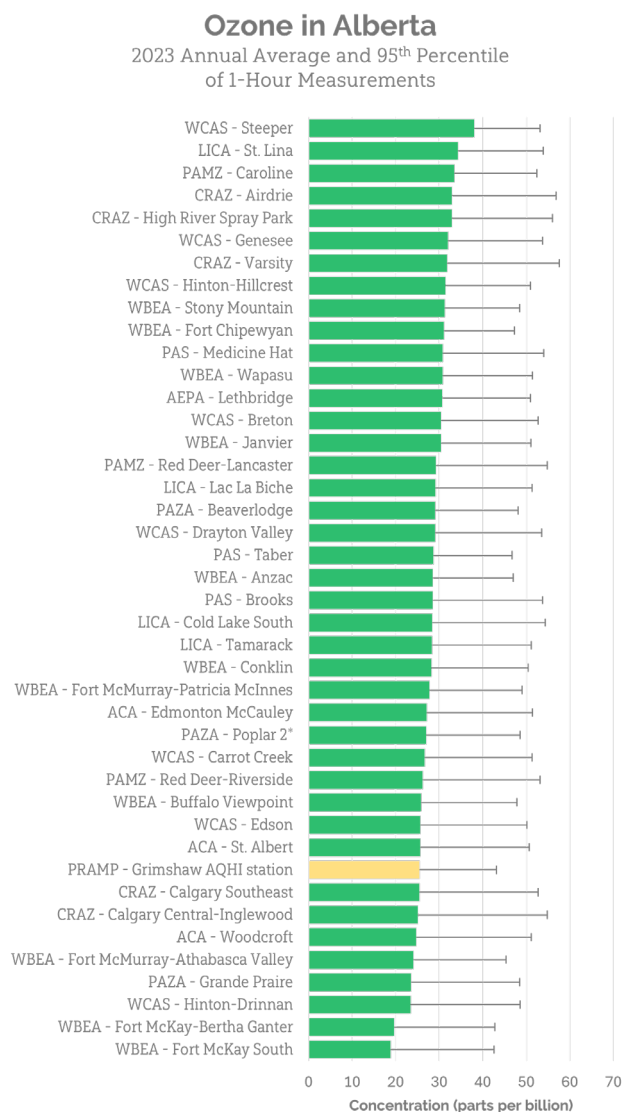
Figure 41: 2023 Ozone in Alberta
