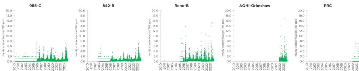
Figure 26: 2010-2023 Hourly total reduced sulphur compounds concentrations
