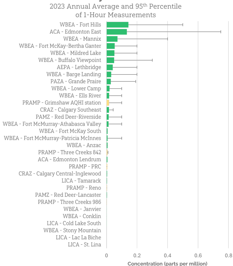
Figure 11: 2023 Non-methane hydrocarbons in Alberta
