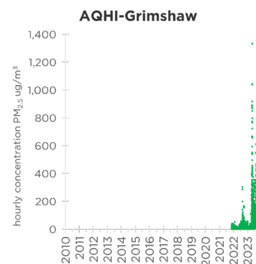
Figure 50: 2010-2023 Hourly particulate matter concentrations
