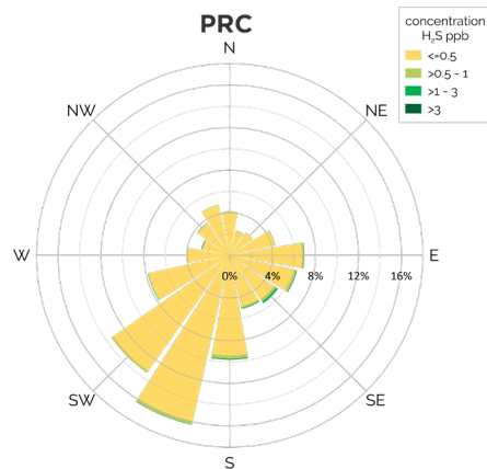
Figure 31: 2023 Hourly hydrogen sulphide concentration wind rose
