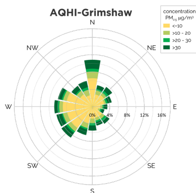
Figure 49: 2023 Hourly particulate matter concentration wind rose
