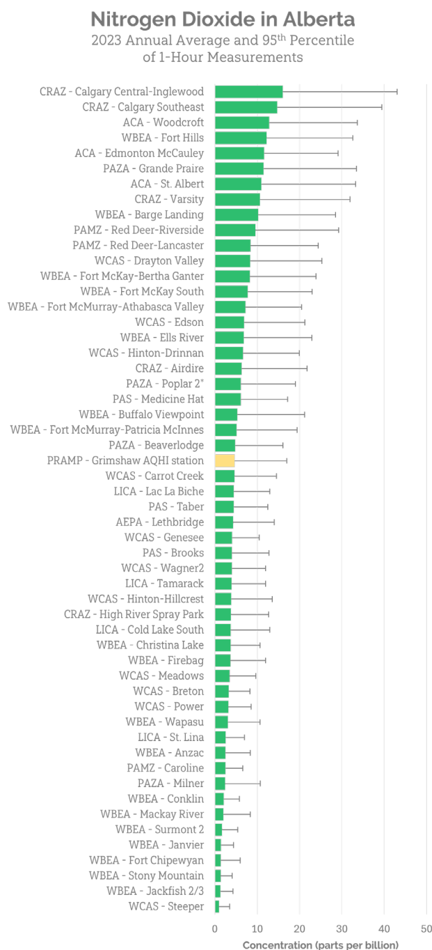
Figure 35: 2023 Nitrogen Dioxide in Alberta
