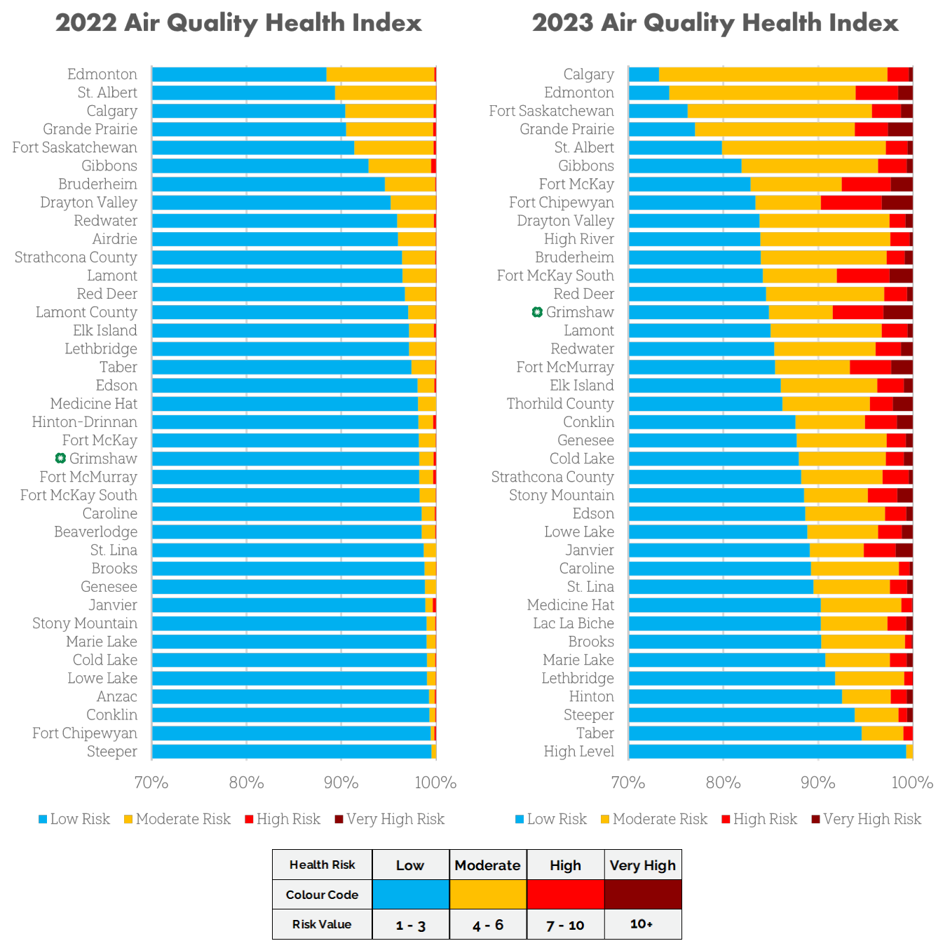
Figure 53: Comparison between 2022 and 2023 Air Quality Health Index values in Alberta
