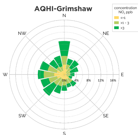
Figure 38: 2010-2023 Hourly nitrogen dioxide concentrations
