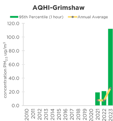
Figure 51: 2010-2023 Annual averages and 95 th percentile of hourly measurements of particulate matter
